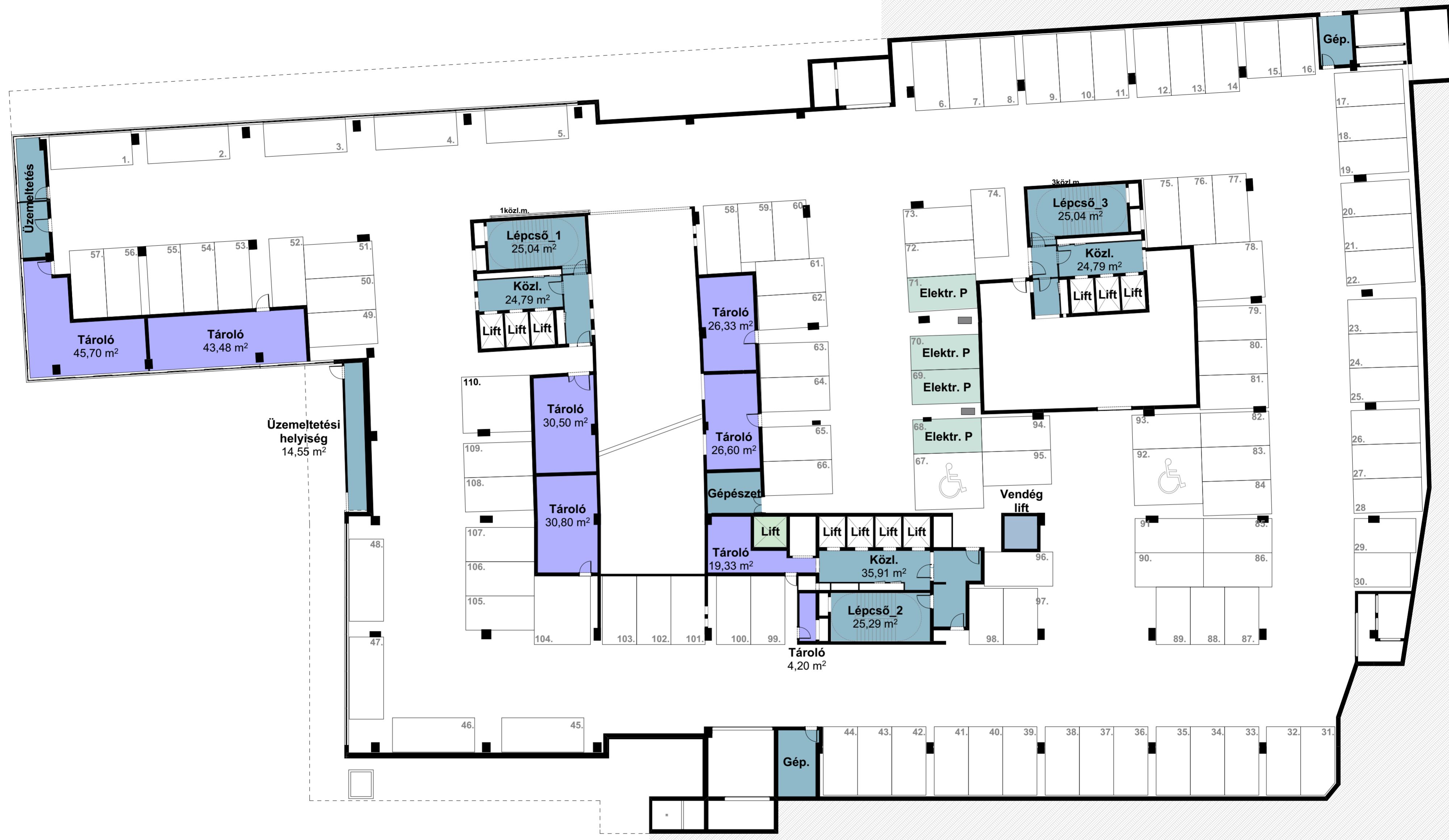
-1st Basement M1:200
