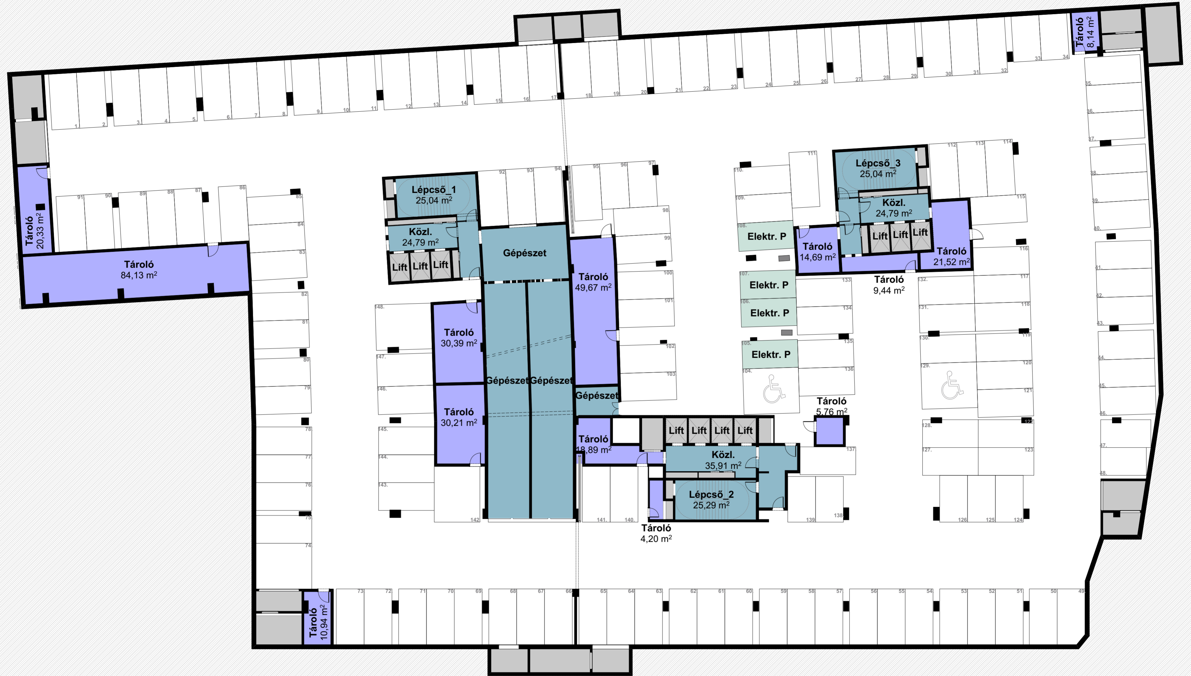
-3rd Basement M1:200
